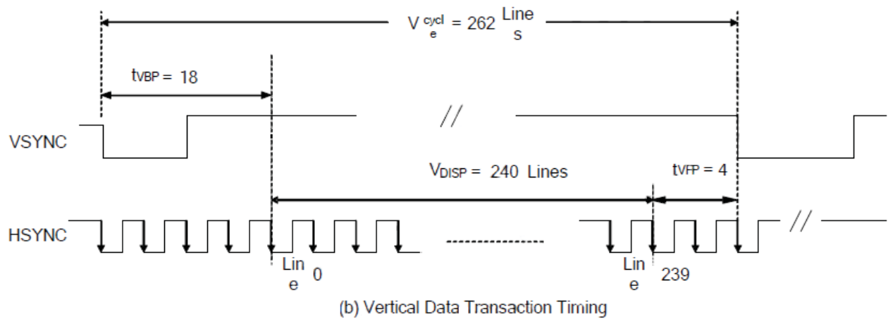
Figure 4: Data Transaction Timing in Parallel RGB (24Bit) interface (SYNC Mode)
