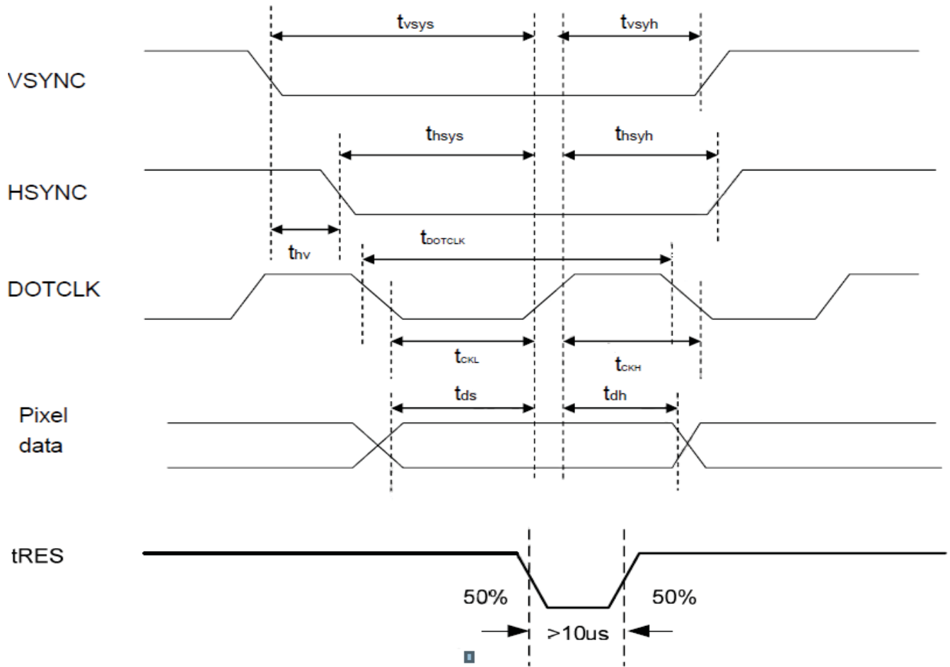
Figure 3: Pixel Timing
